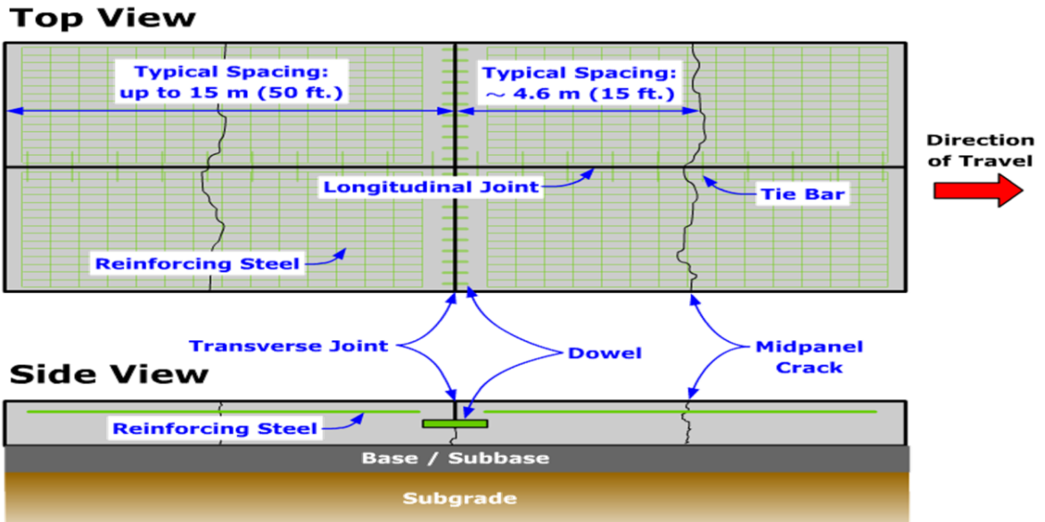
Figure 13 Top View and Side View of Jointed Reinforced Concrete Pavement
