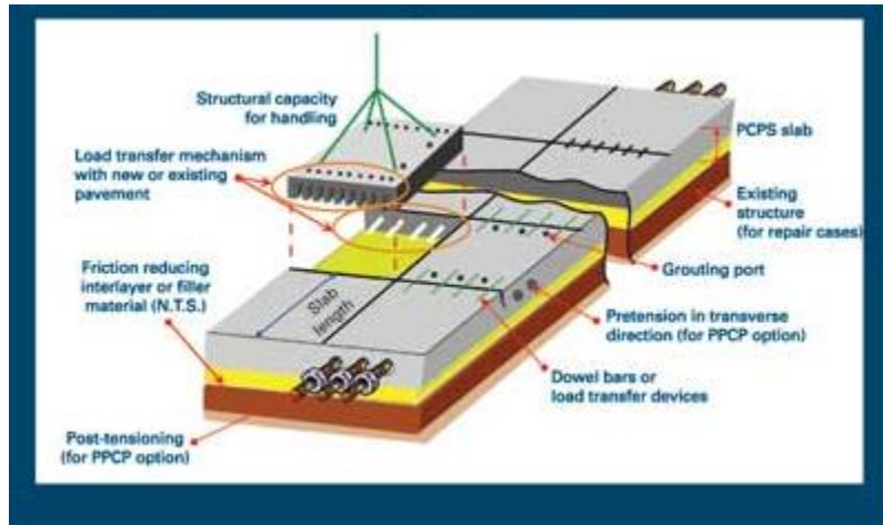
Figure 15 Precast Concrete Pavement Components
