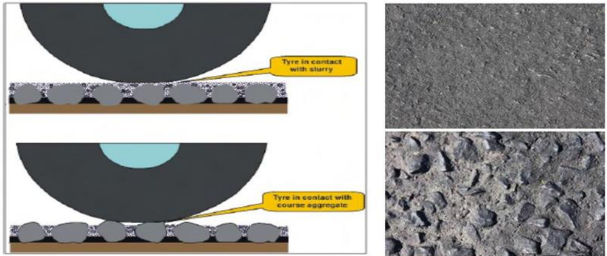
Figure 62 Cape Seal
