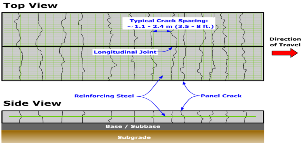
Figure 14 Top View and Side View of Continuously Reinforced Concrete Pavement
