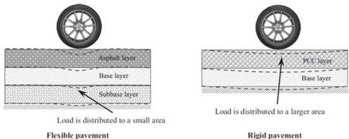
Figure 3 Deformation Behaviour of Flexible and Rigid Pavements
